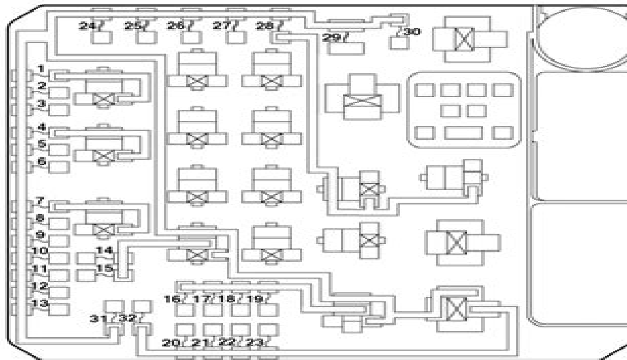
Relay box
