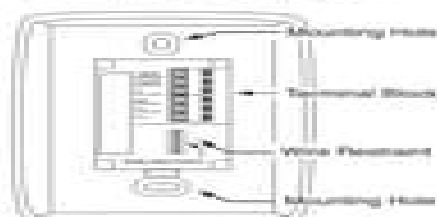
FG-1625F Glassbreak Detector, Back View
