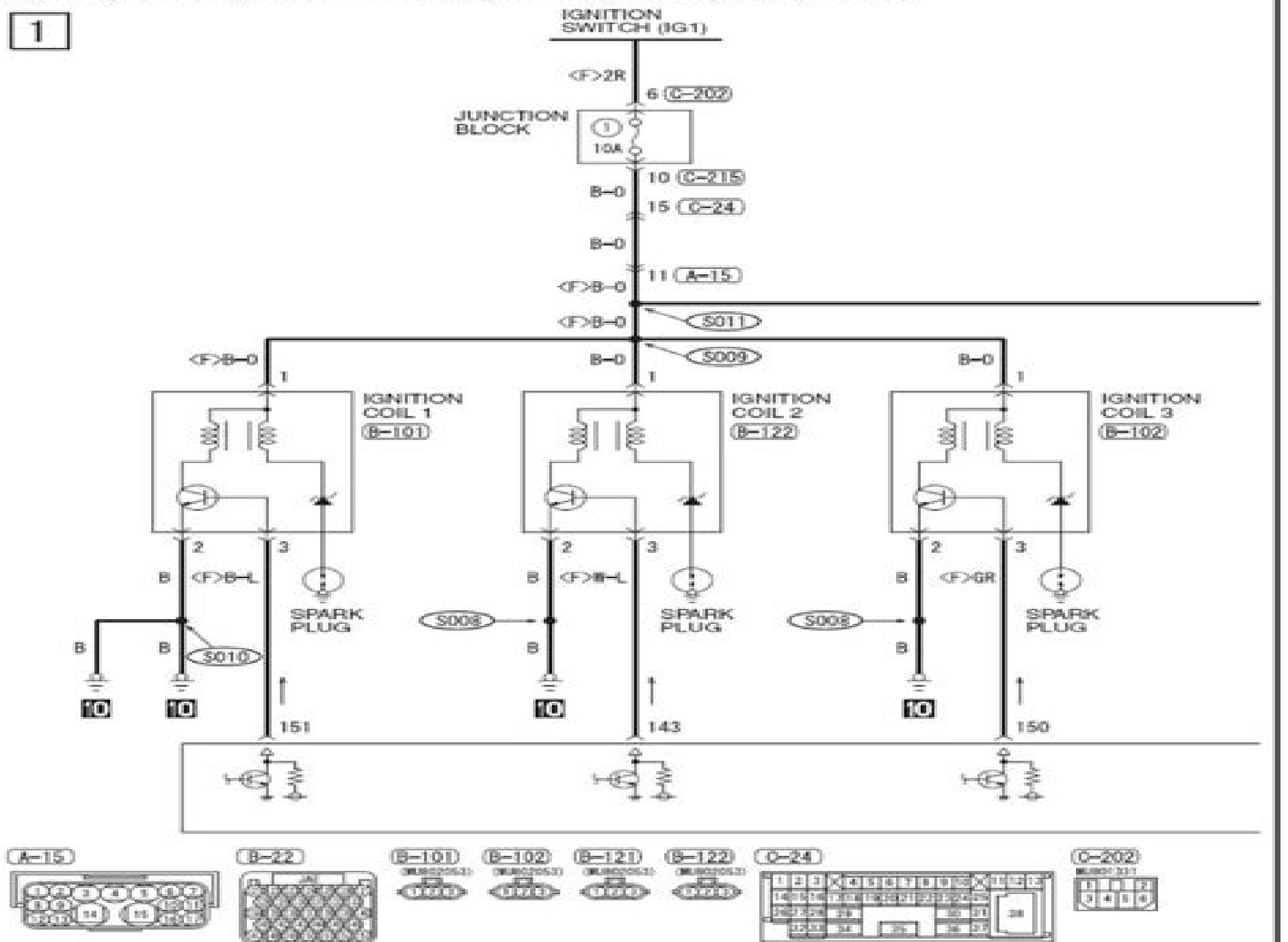
Fig 1: Ignition System - 2.4L Engine Circuit Diagram (1 Of 2)
