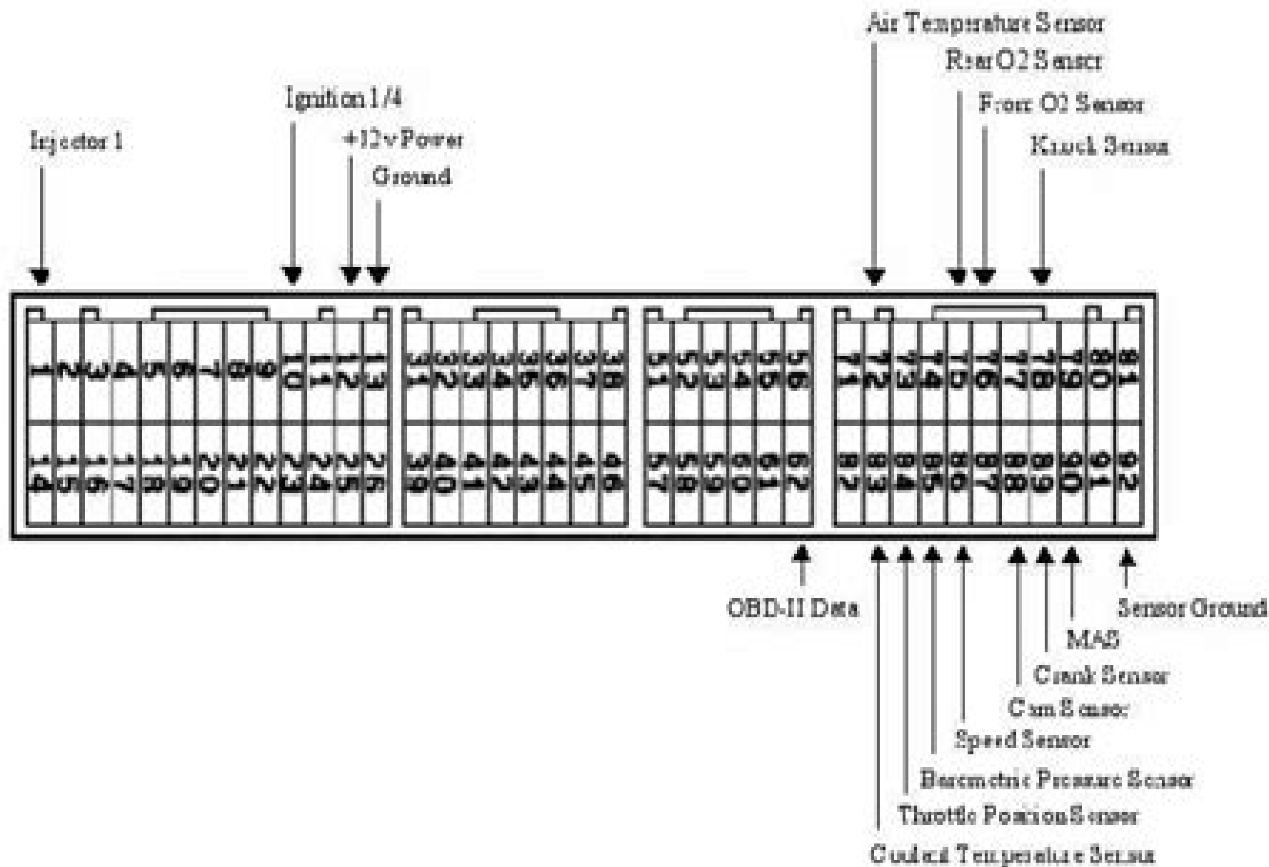
Illustration 4- The second generation DSM and EVO VIII ECU pinout
