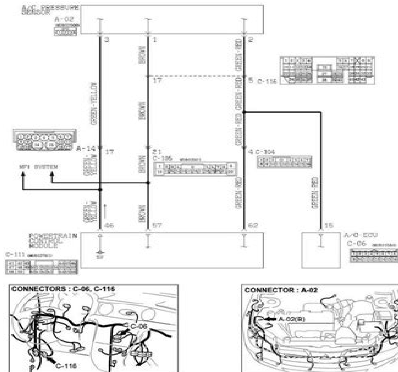
Fig. 110: A/C Pressure Sensor Circuit Diagram Courtesy of MITSUBISHI MOTOR SALES OF AMERICA.
