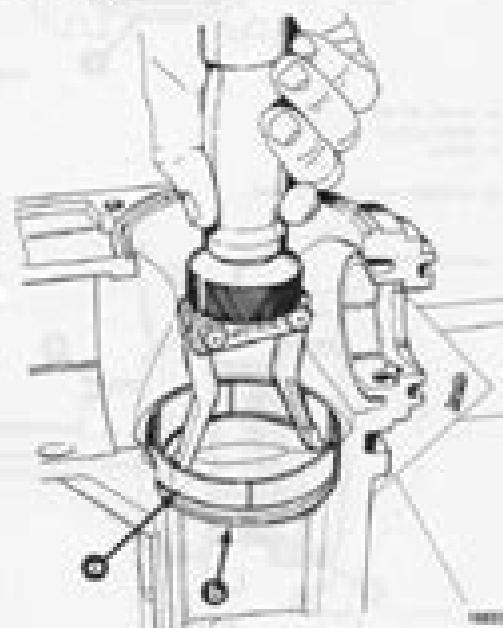
a - Bearing Cap b - Shim
