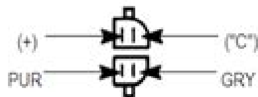
IGNITION COIL CONNECTOR
