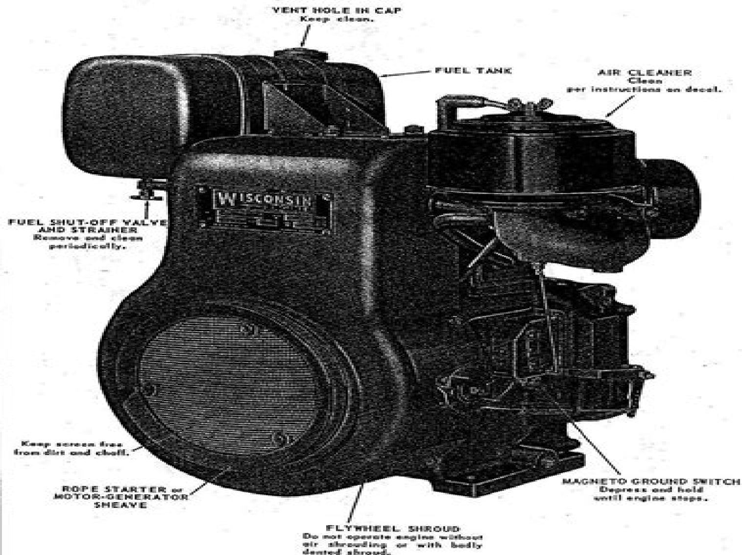
Fig. 2 FAN END (front) and RIGHT HAND SIDE VIEW of ENGINE
