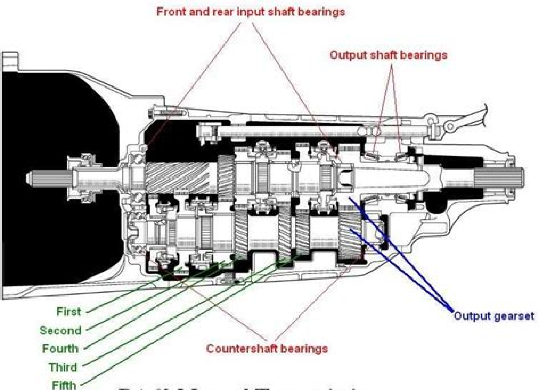
RA62 Manual Transmission
