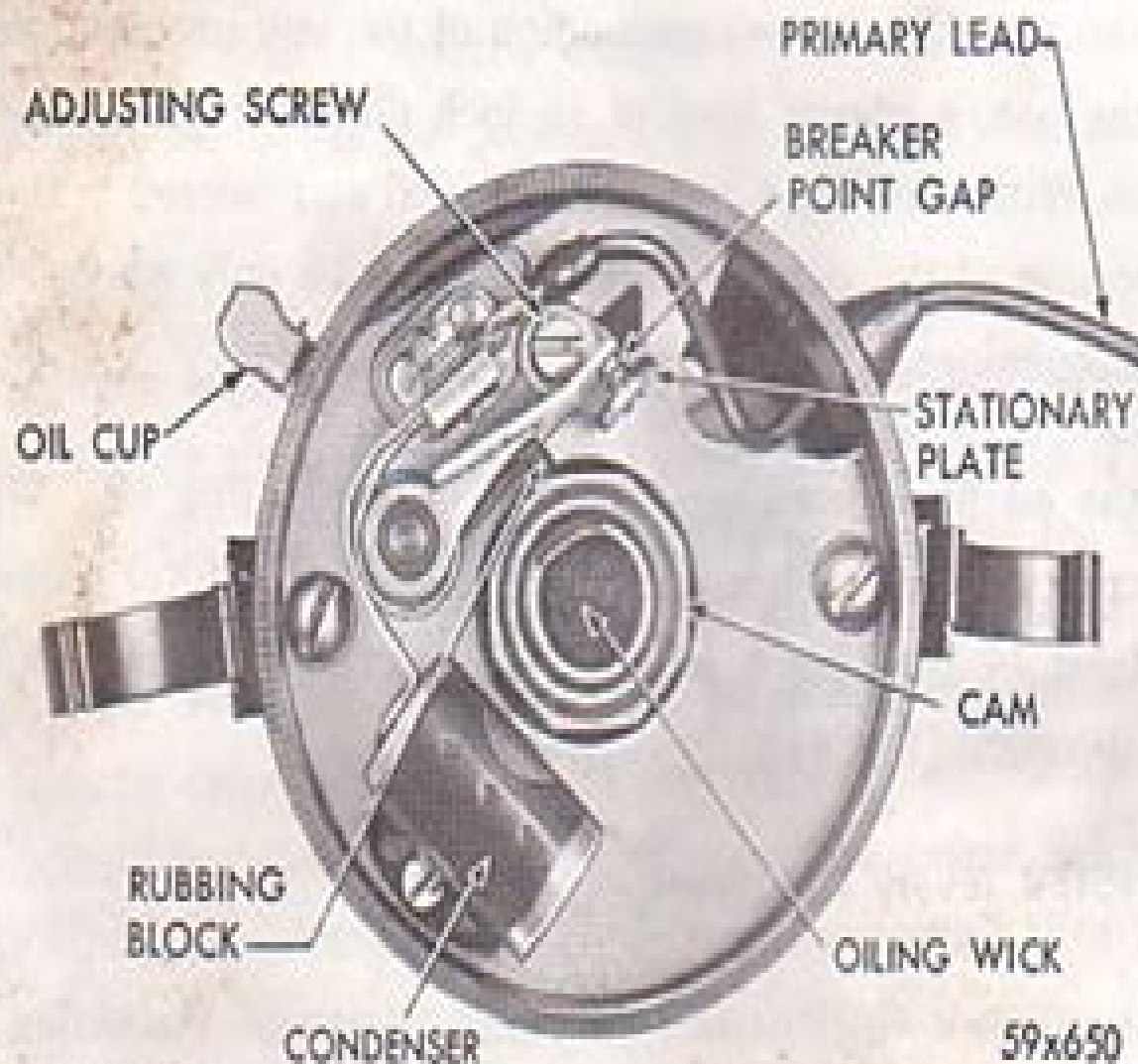
Figure 43—Distributor Lubrication Points
