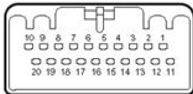
Device Connector(20P)
