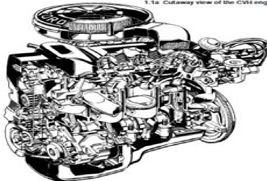
1.1a Cutaway view of the CVH engine
