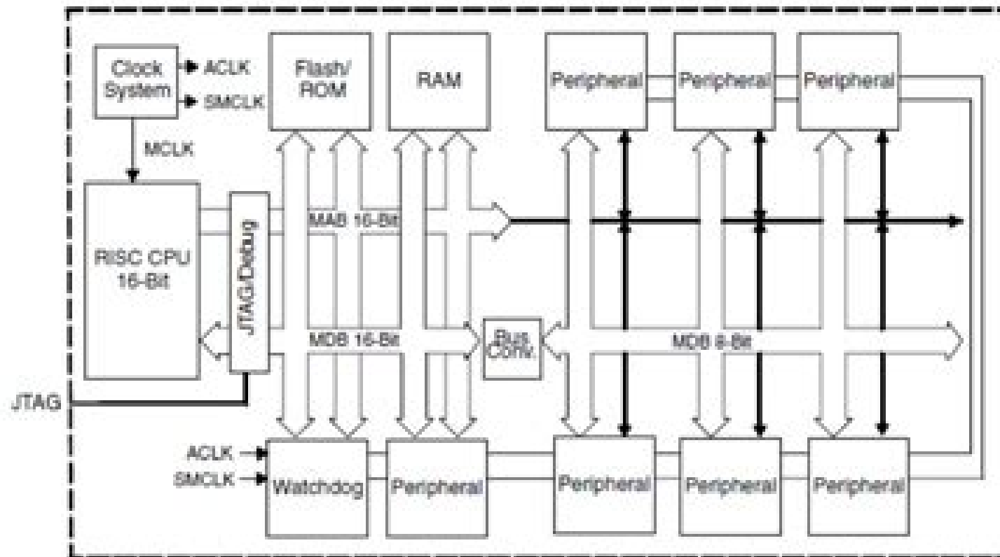
Figure 1-1. MSP430 Architecture
