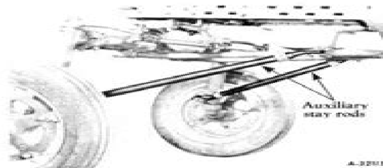
Illustr. 93 Farmall 300 Hi-Clear with auxiliary stay rods.
