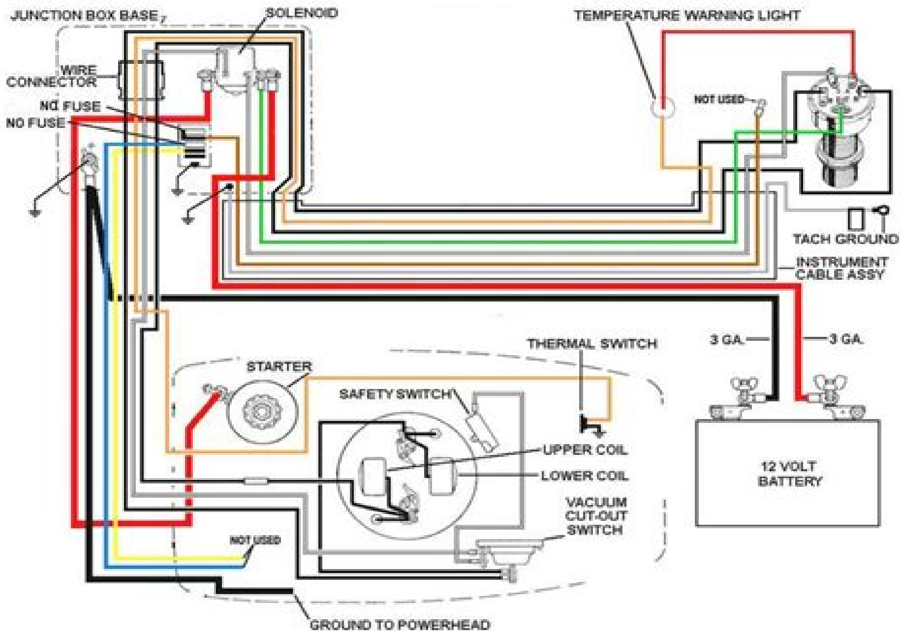
WIRING DIAGRAM 1962-63 40hp WITHOUT GENERATOR
