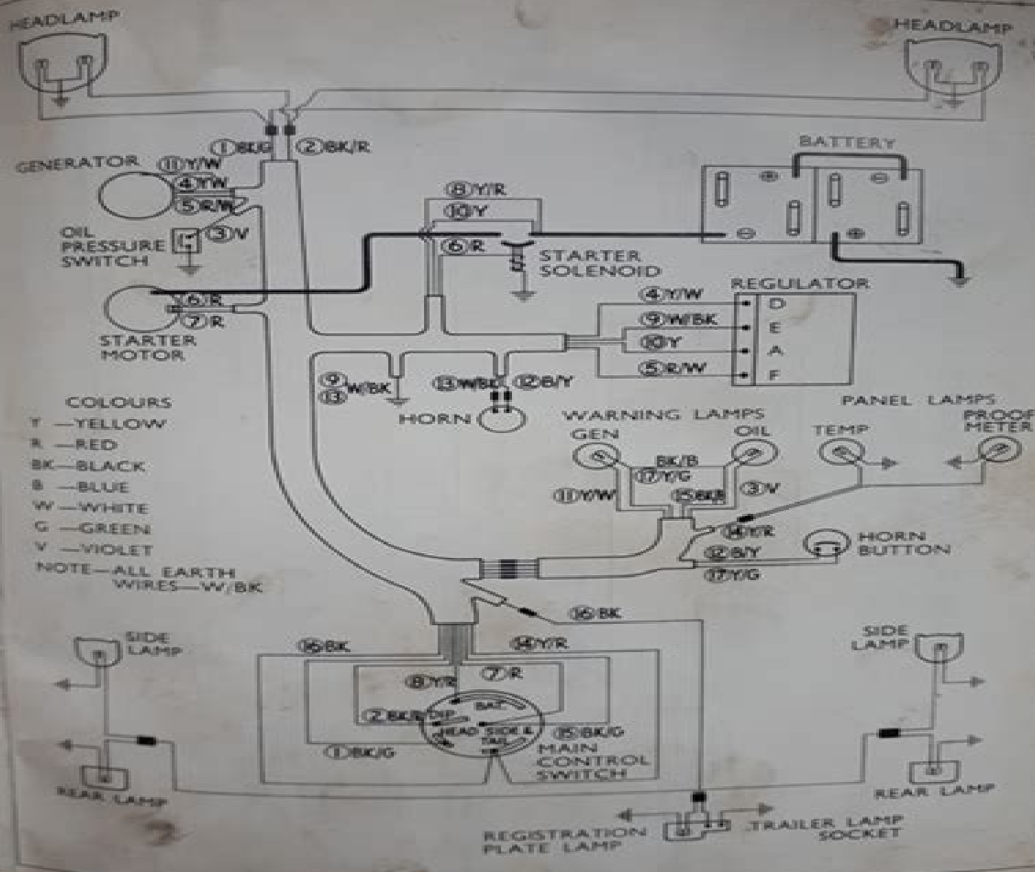
Fig. 27. Diesel Tractor Wiring Diagram (except Inertia Starter)
