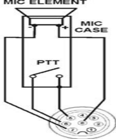
TRANSCEIVER MICROPHONE JACK FRONT VIEW
