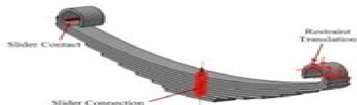
Fig. 2 Boundary condition of MLS
