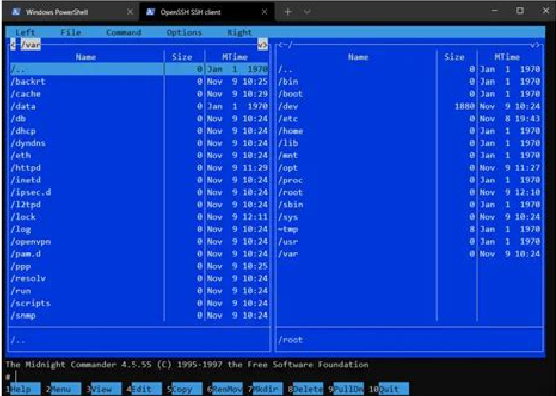
Figure 1: Midnight Commander
