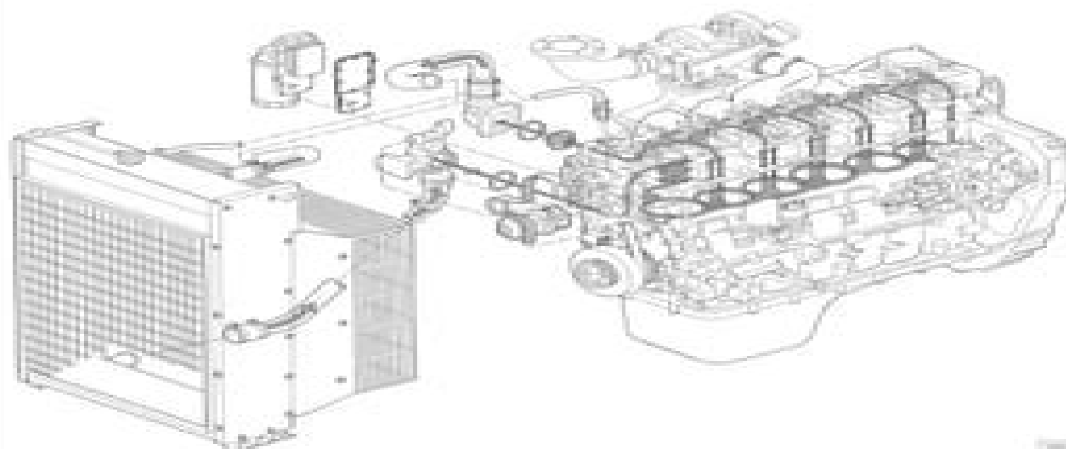
COOLING SYSTEM LAYOUT
