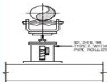
SH_Type_F_PipeRoller_DWG, DXF or EPS
