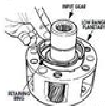
Figure 3-129 Input gear lock ring removal
