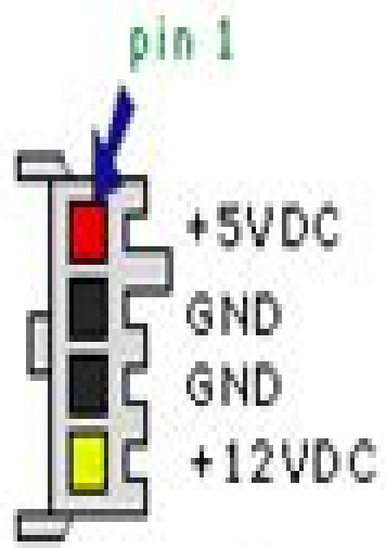
4 pin Berg Floppy Drive Connector
