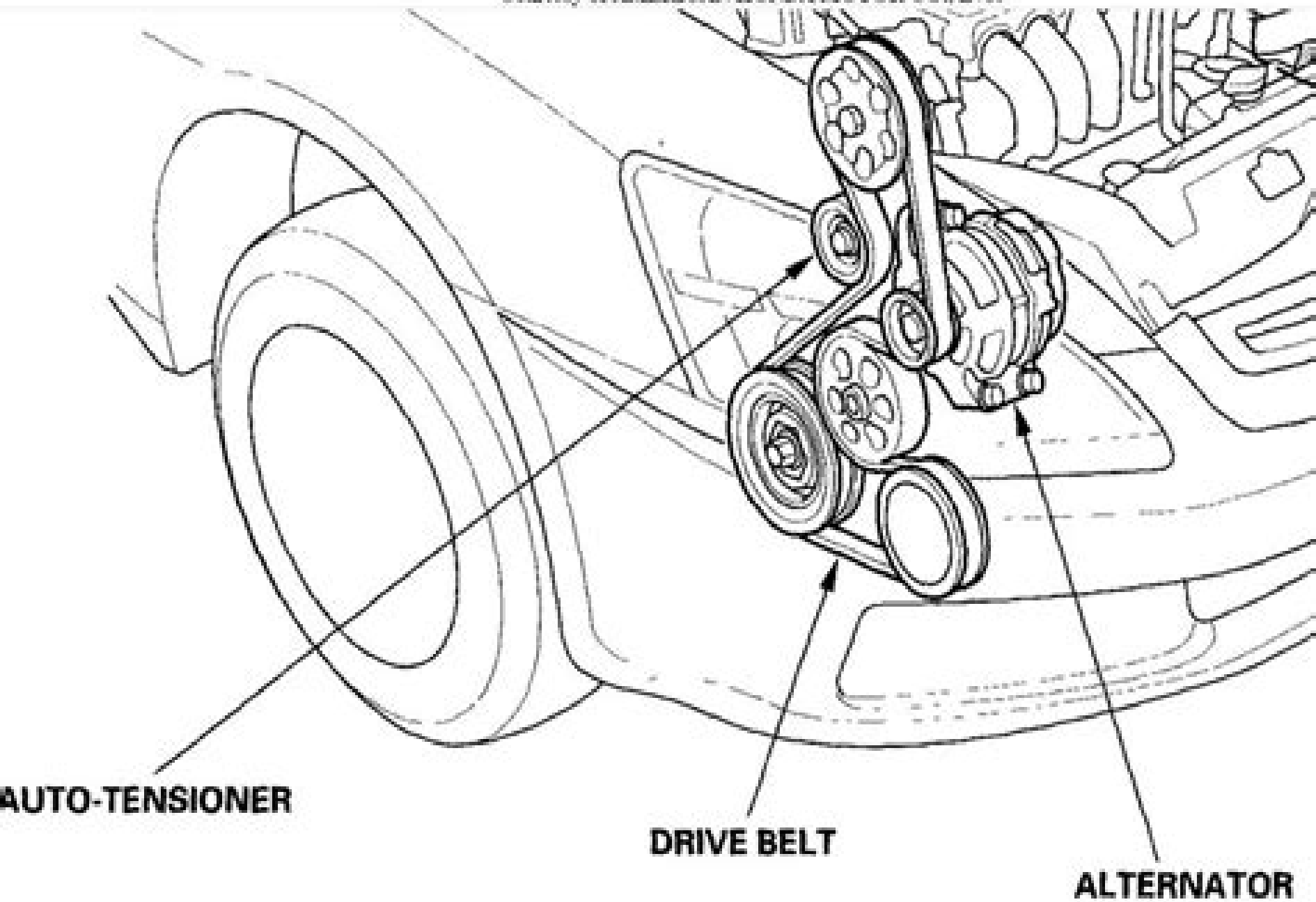
Fig. 1: Identifying Components Of Charging System Courtesy of AMERICAN HONDA MOTOR CO., INC.
