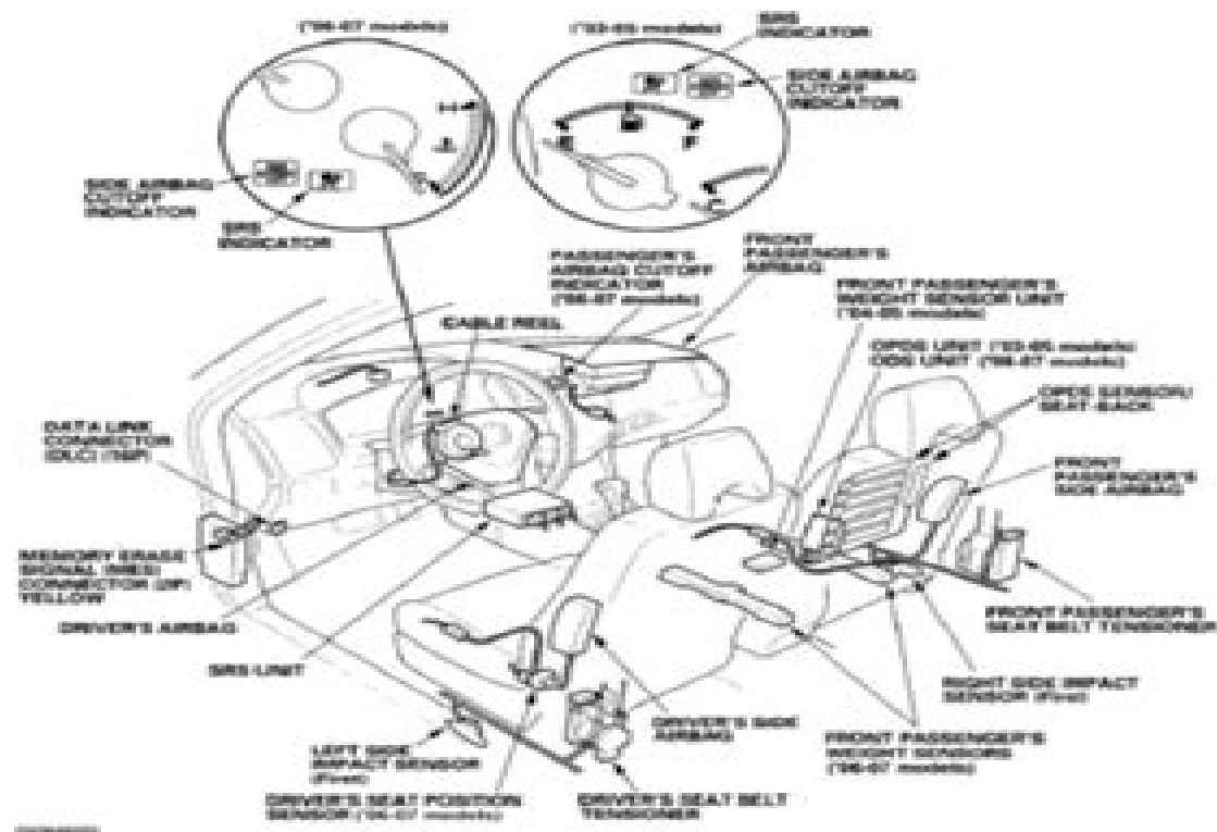
Fig. 1: Locating SRS Components
