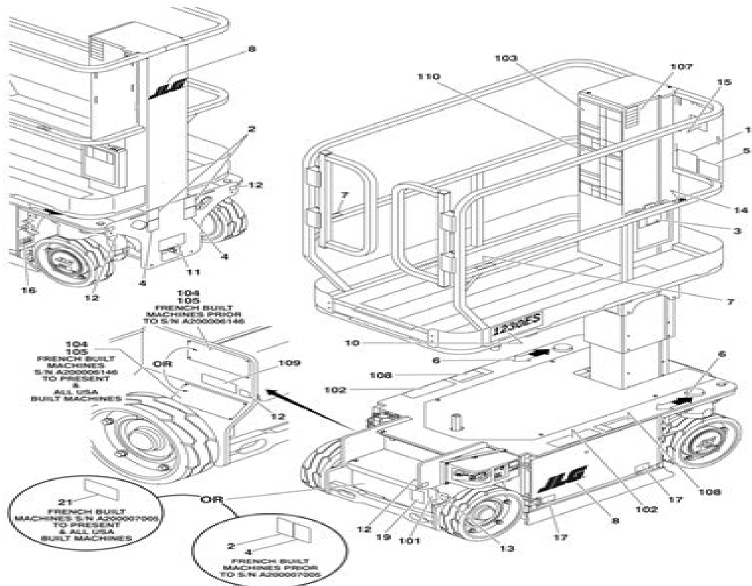
FIGURE 8-1. DECAL INSTALLATION
