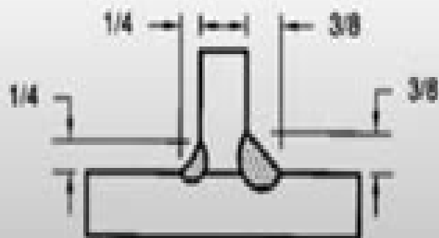
WELD CROSS SECTION
