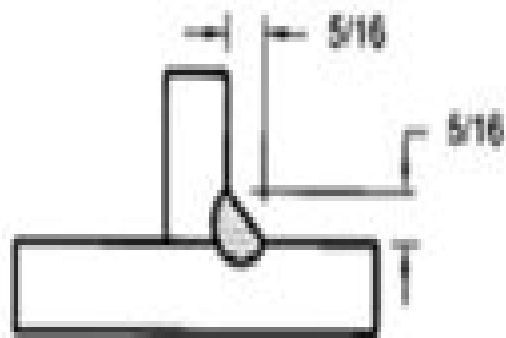
WELD CROSS SECTION
