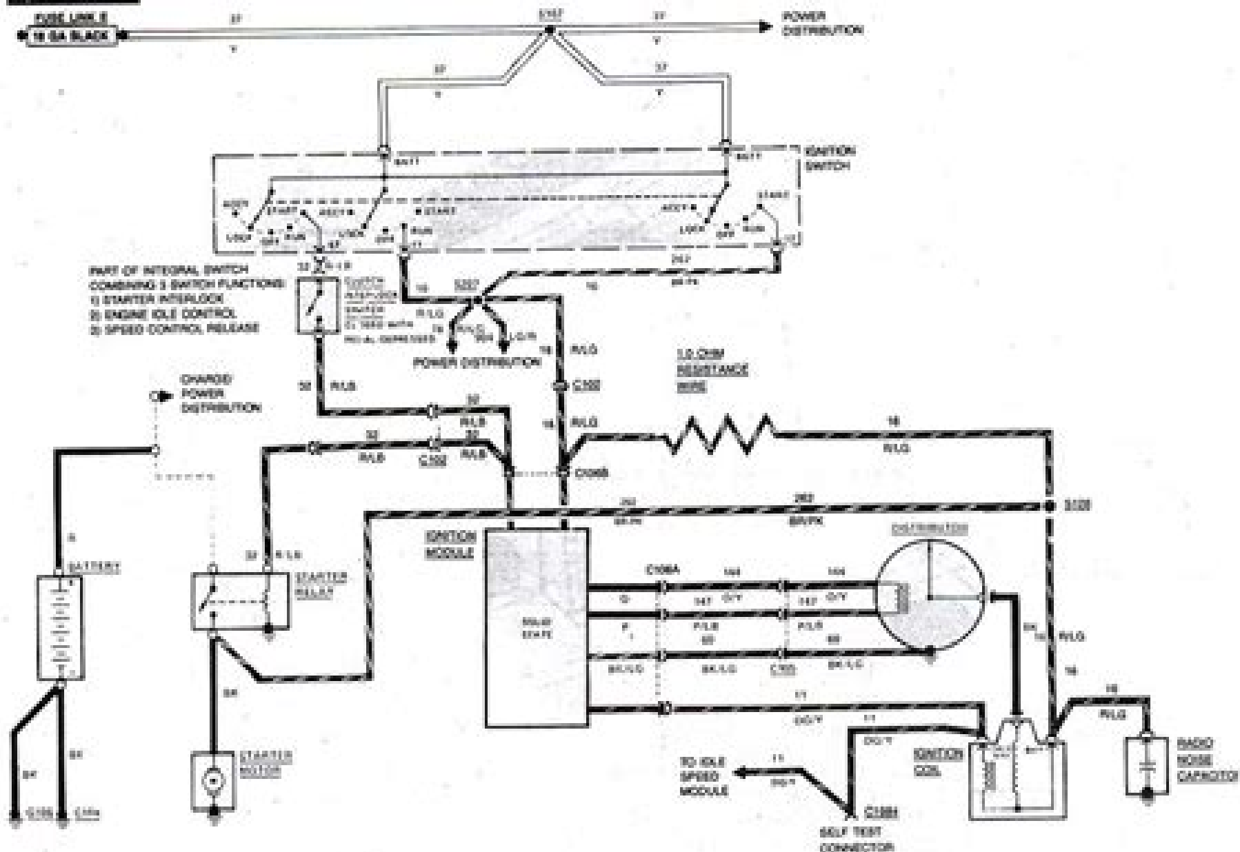
Start/ignition - 2.0L engine (typical)
