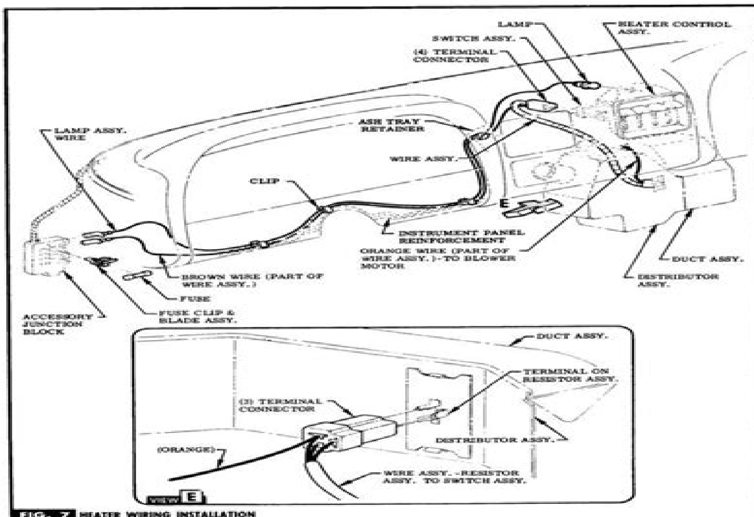
FIG. 7 HEATER WIRING INSTALLATION
