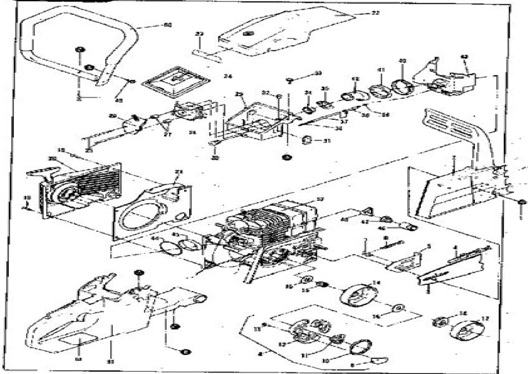
Figure 1 GENERAL ASSEMBLY
