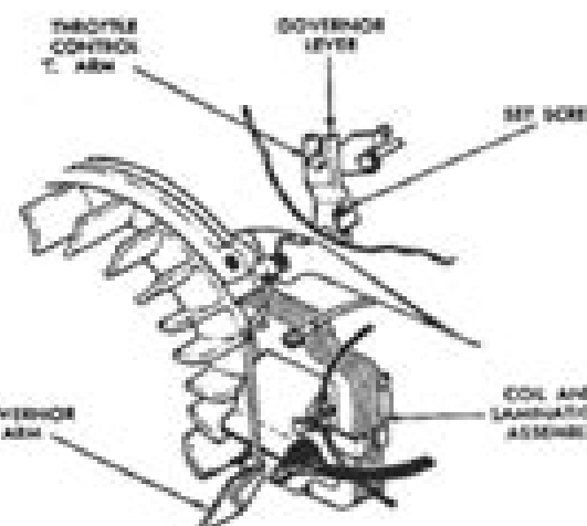
Fig. MC3-7—Typical air vane governor installation on Model 895.
