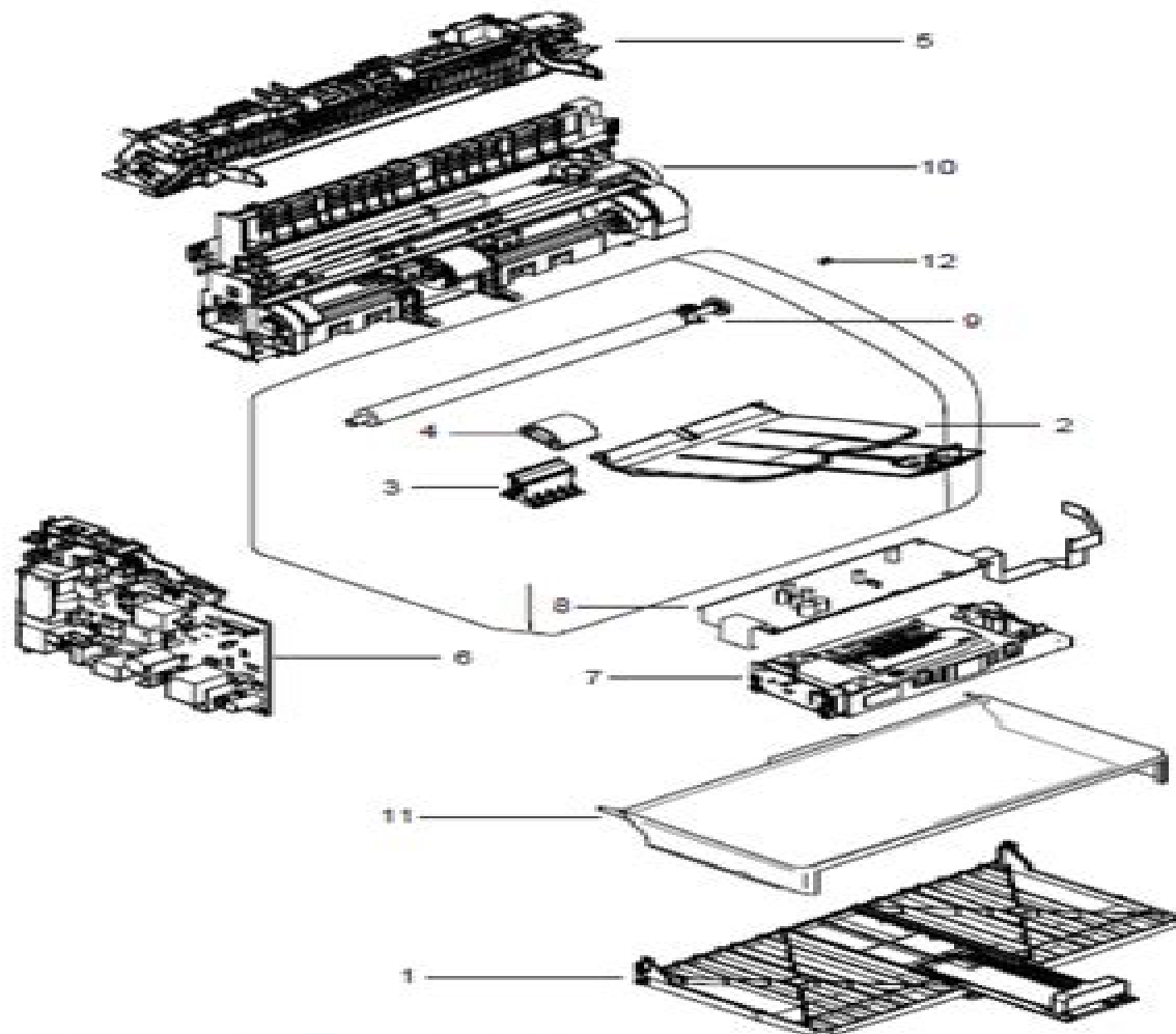
Exploded View: Field Replaceable Units
