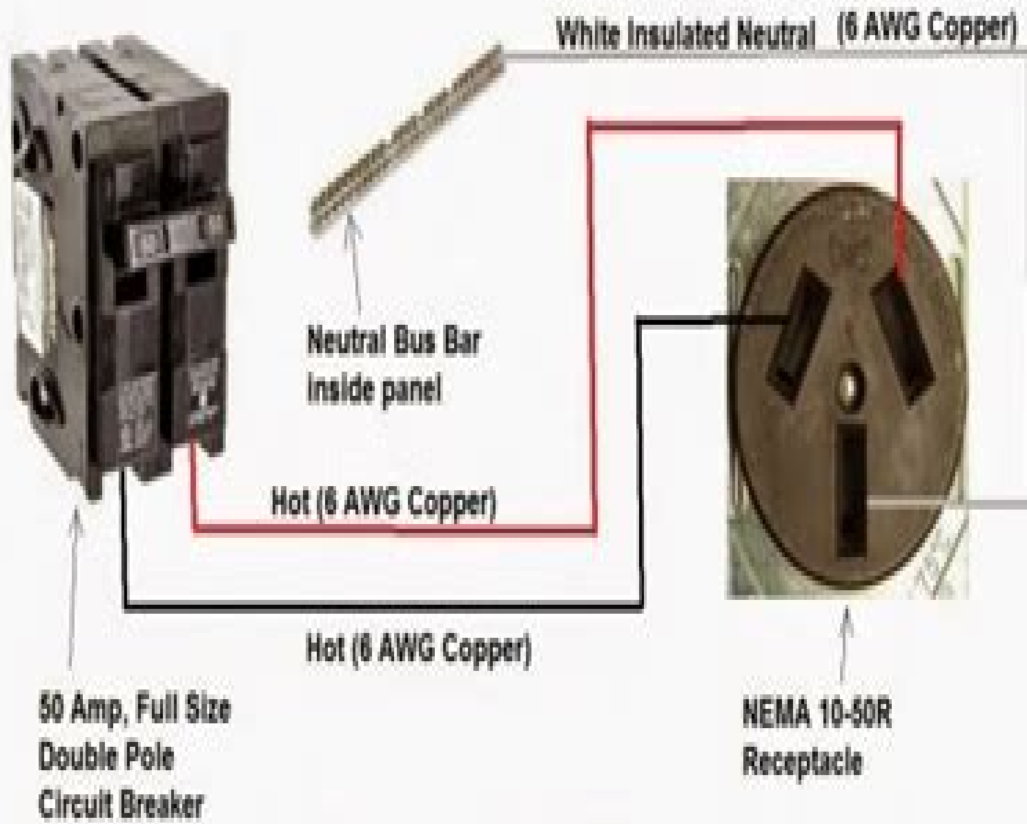
50 Amp, 3 wire Range Circuit
