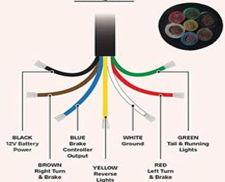
Wiring Side
