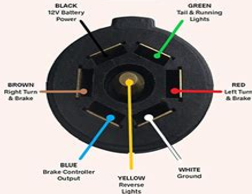
Plug Side
