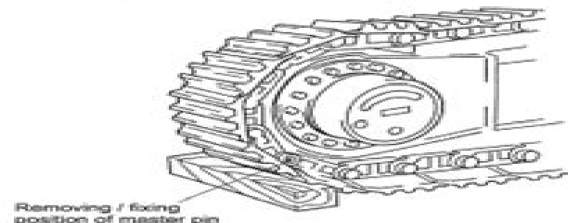
Fig. 34-3 Removing/fixing position of master pin
