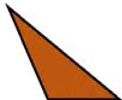
Obtuse triangle
