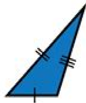
Scalene triangle
