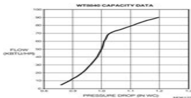
Fig. 1. Typical capacity curve for WT88xx family of water heater control systems.
