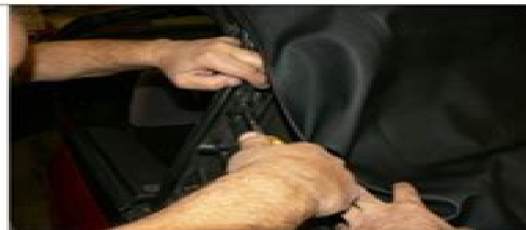
Step 24: CONTINUED. Insert side cables from front of top side pockets and screw in back end with spring to frame.
