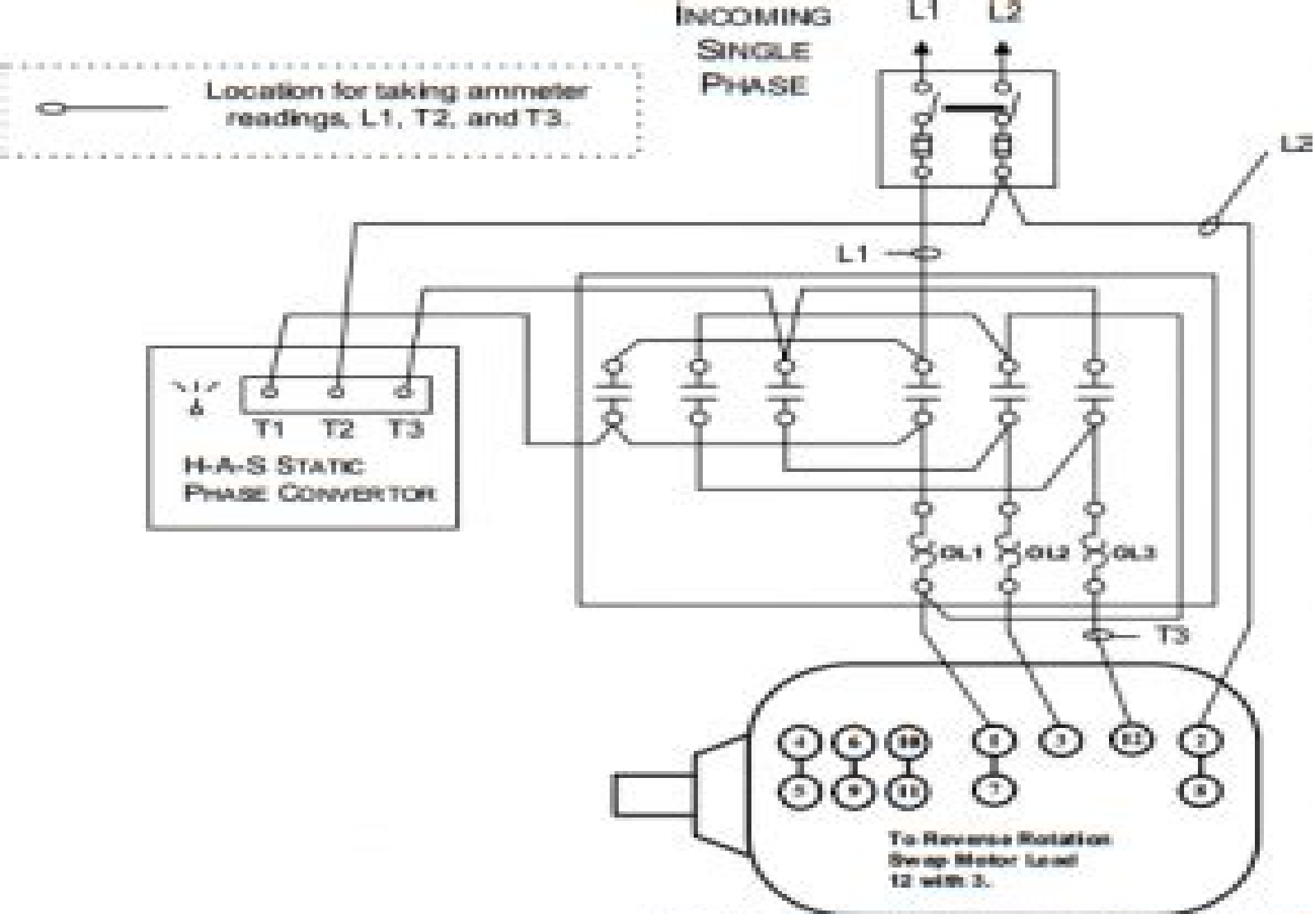
230 Volt Connection of NEMA 12 Lead 230/460 Volt WYE CONNECTED Three Phase Motor (Use with 230 Volt H-A-S Static)
