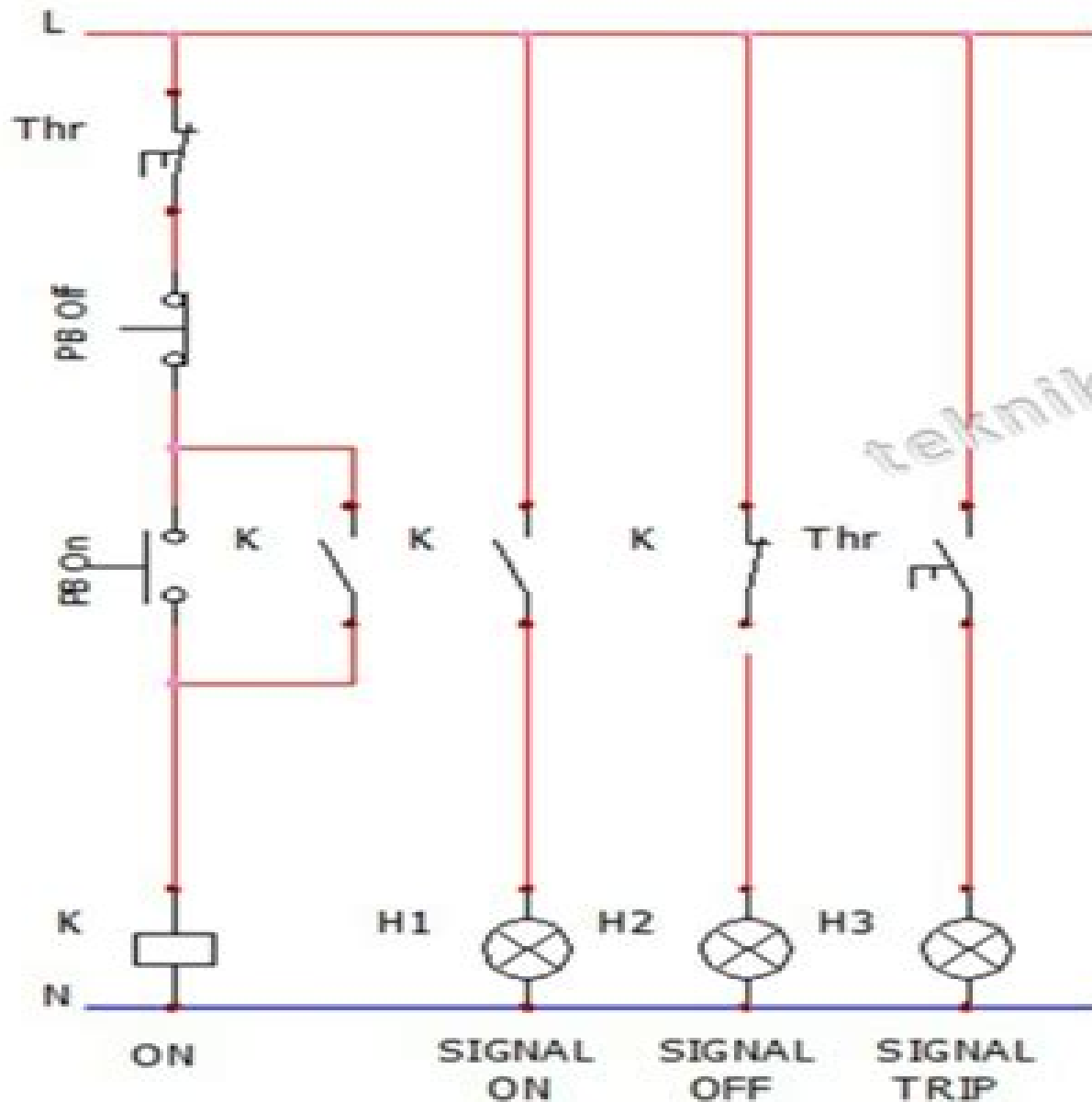
Rangkaian Control
