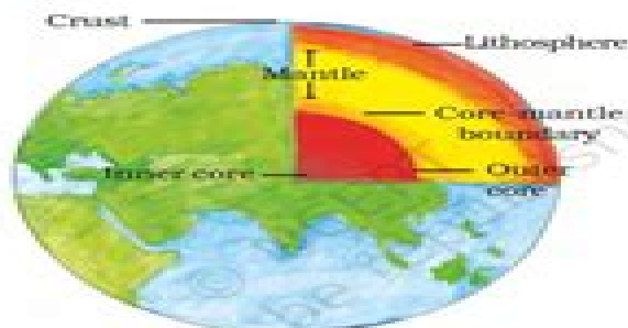
Fig. 2.1: Interior of the Earth
