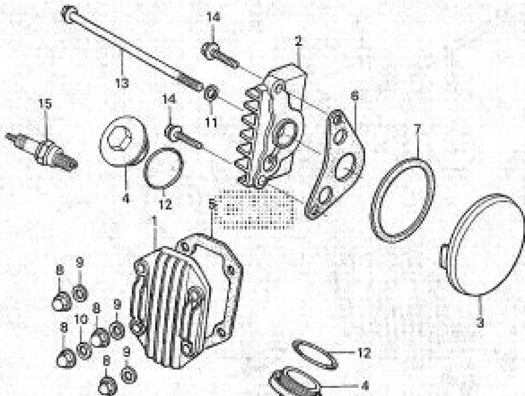
E-1 CYLINDER HEAD COVER
