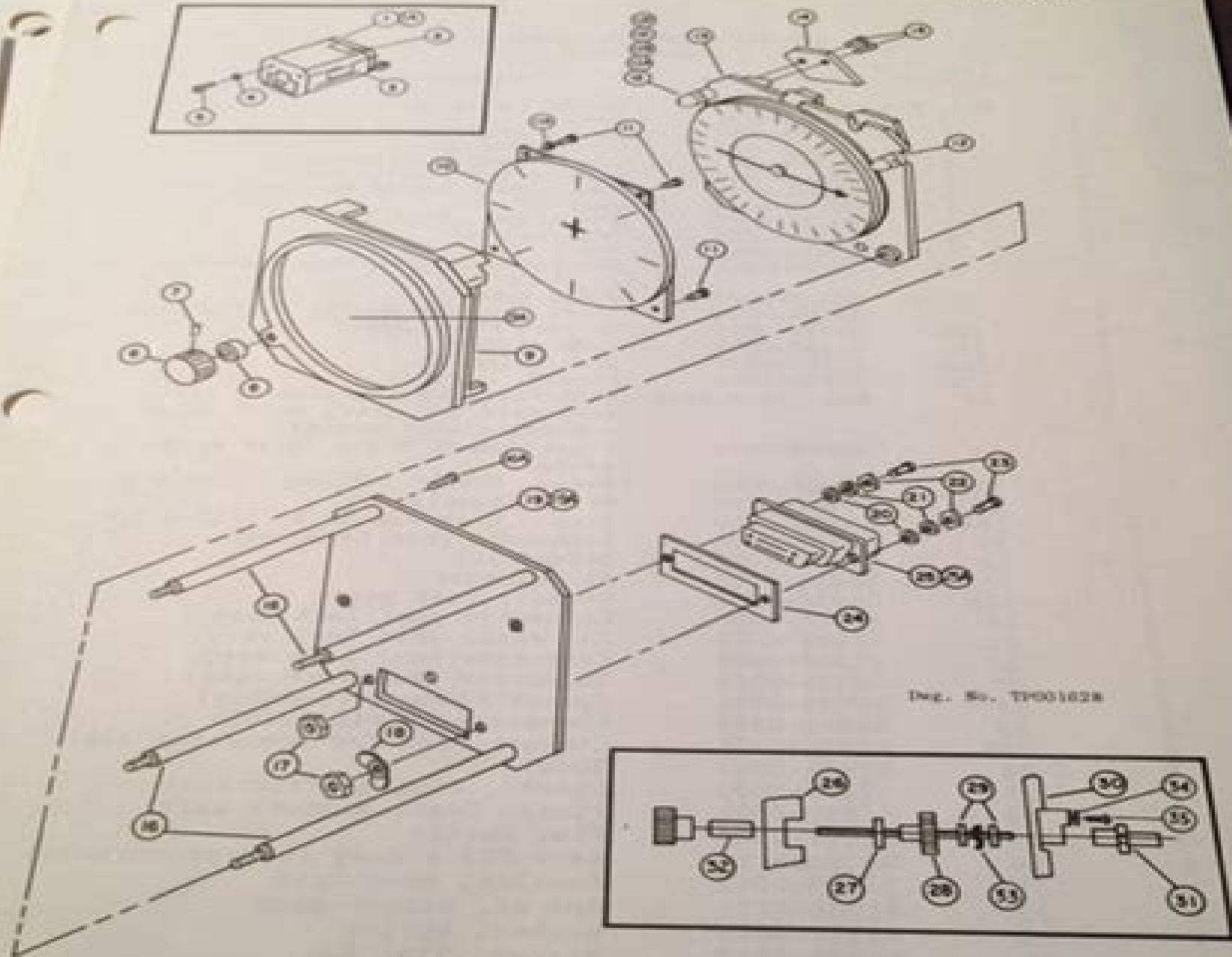
FIGURE 6-6 ID-841 INDICATOR
