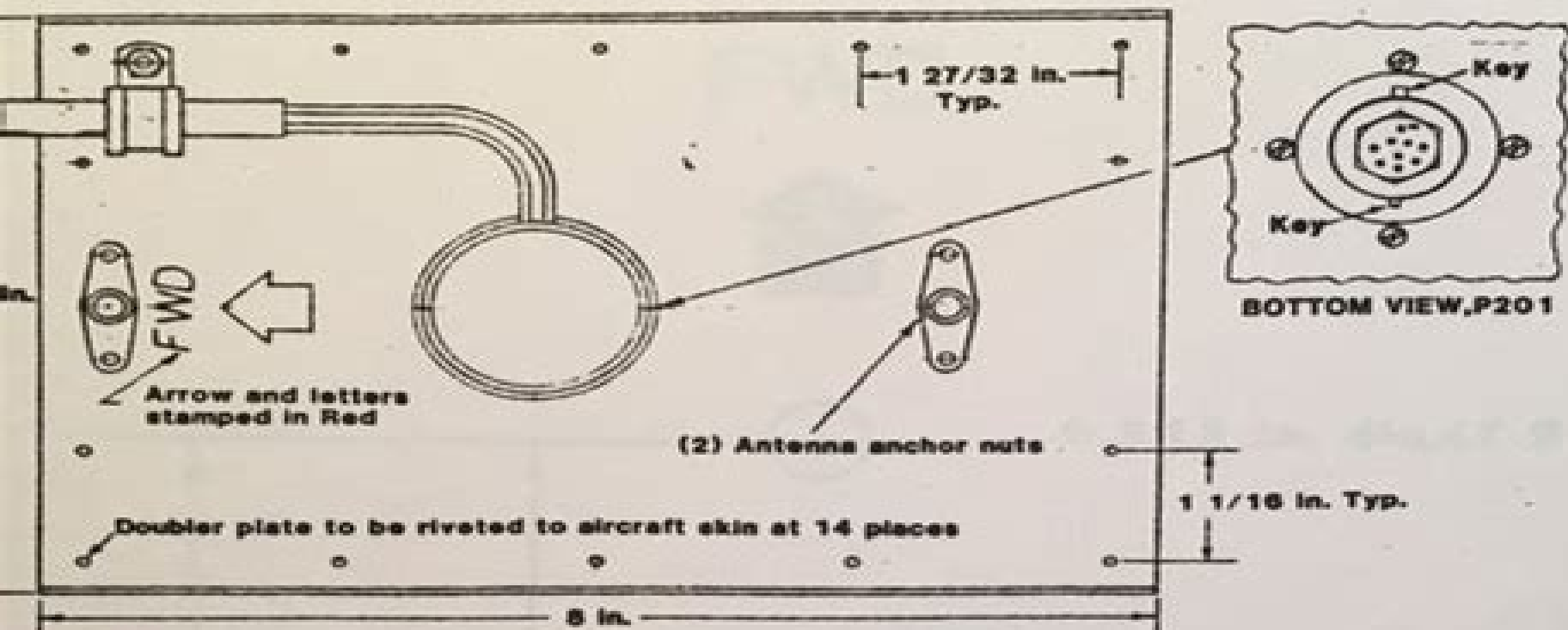
BOTTOM VIEW,CABLE AND ANTENNA DOUBLER PLATE
