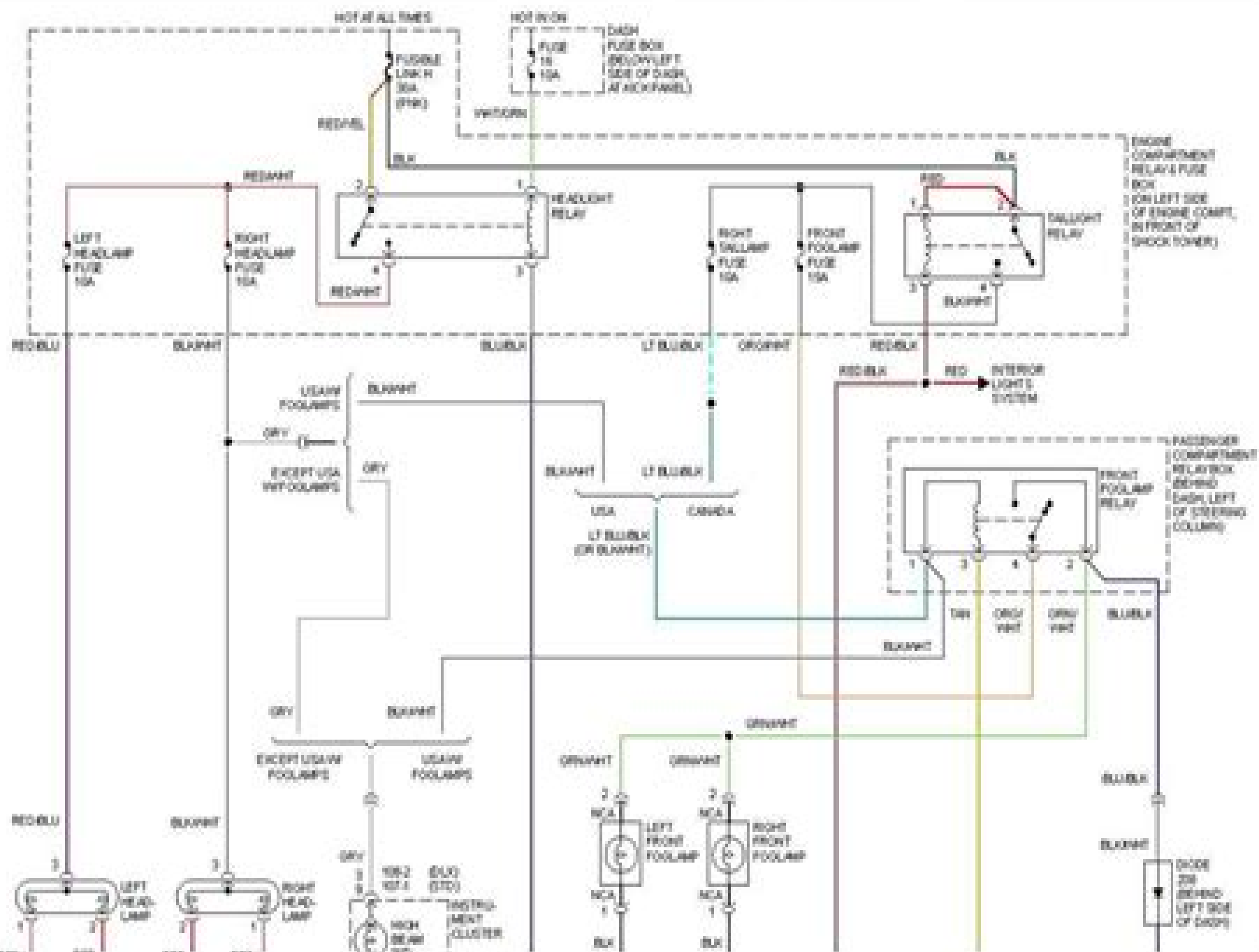
1999 Hyundai Accent GL-Fig. 1: Headlight System Wiring Diagram (Accent)
