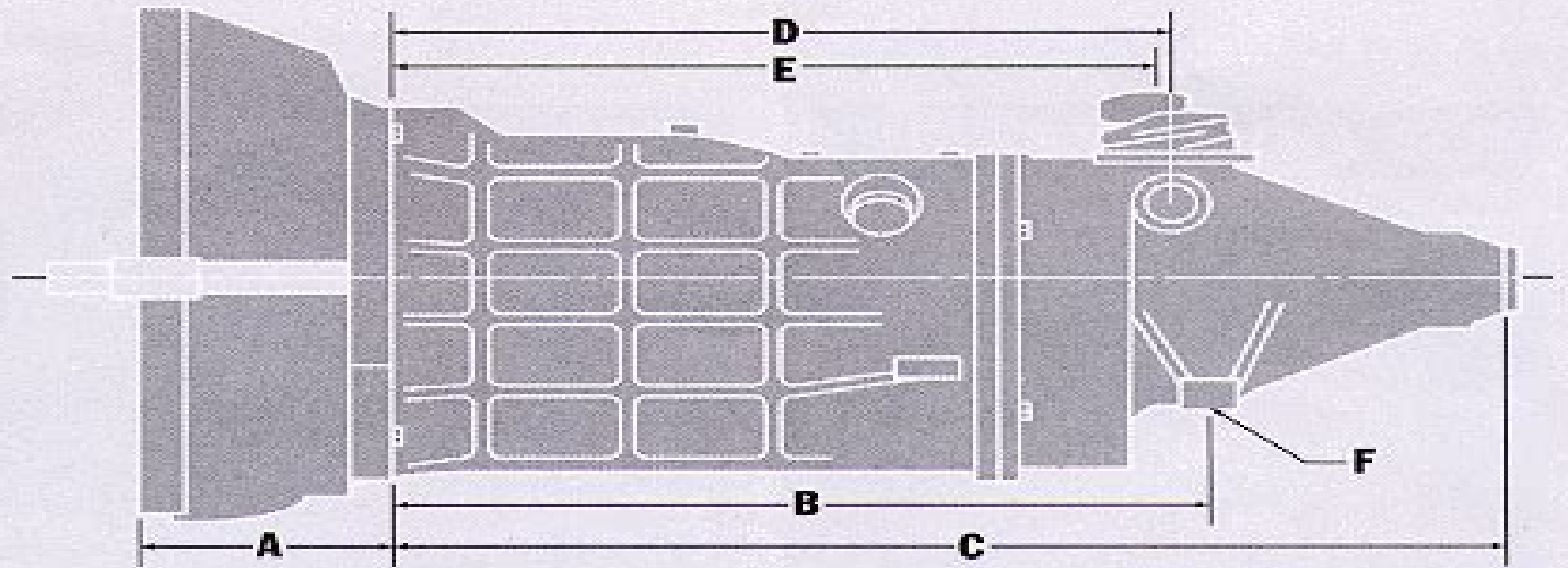
Borg-Warner T56 Six-Speed
