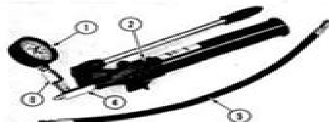
Fig. 9 - Example of Fabricated Hand Tester
