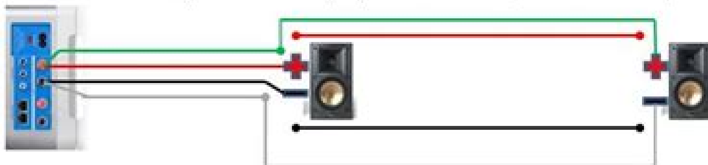
Two Speakers in Parallel (only one channel shown, two conductor cable)
