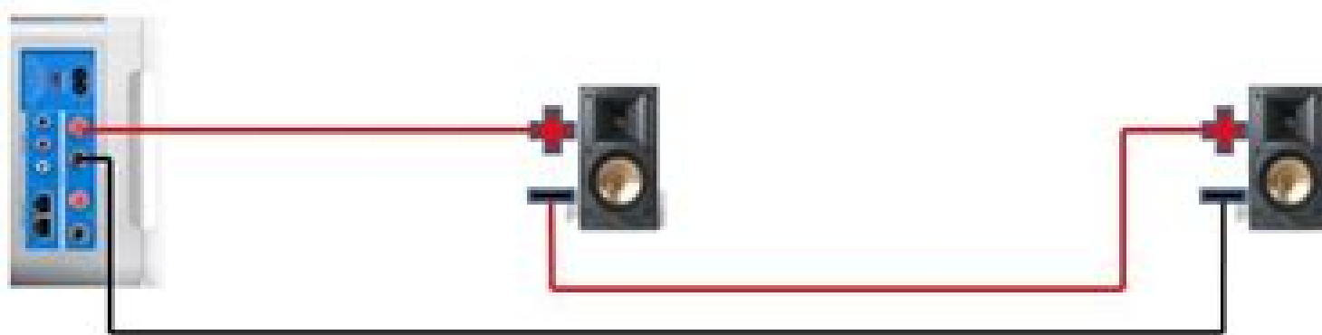
Two Speakers in Series (only one channel shown)
