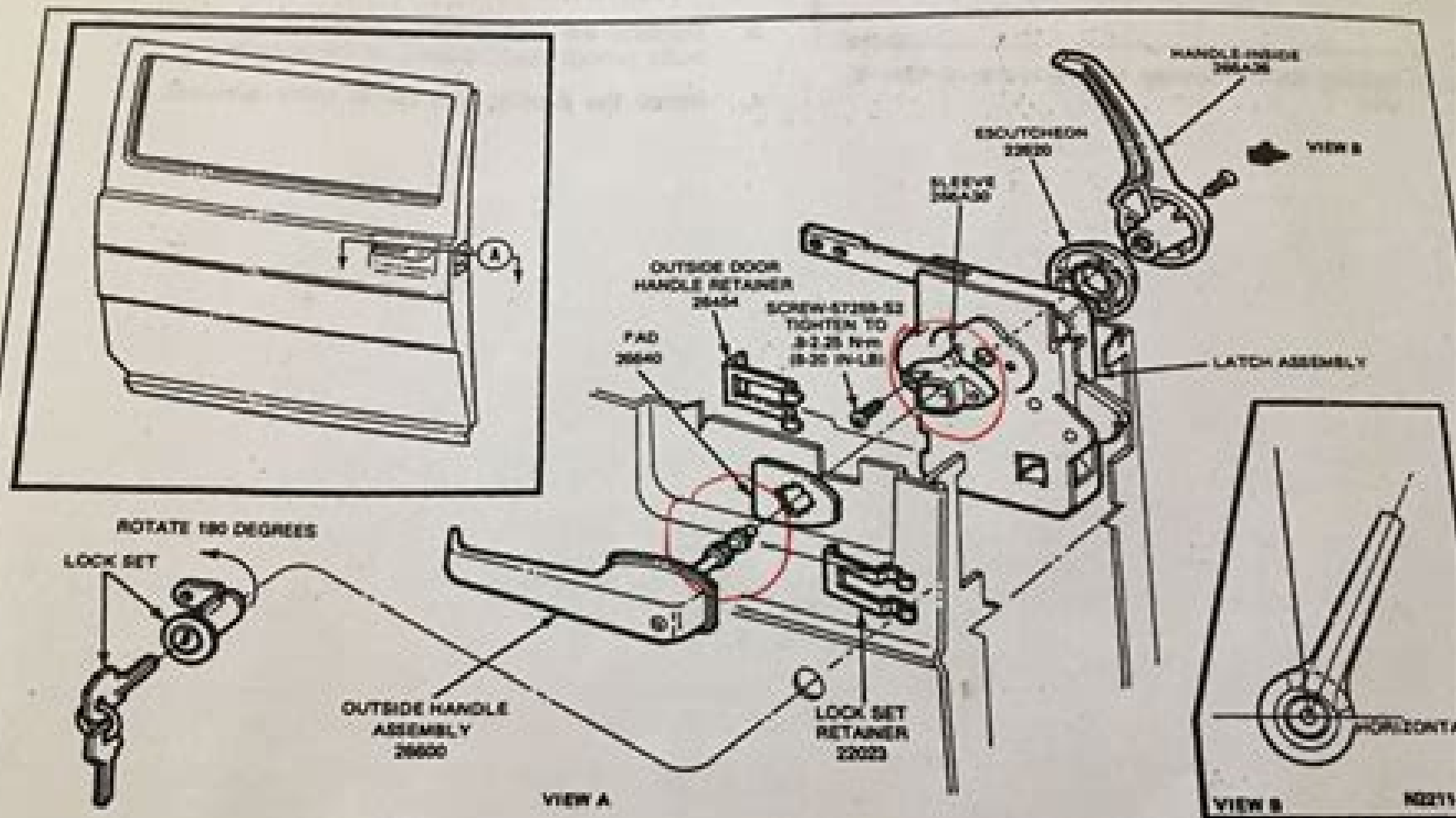
FIG. 5 Sliding Door—Lock and Latch—E-150—E-350
