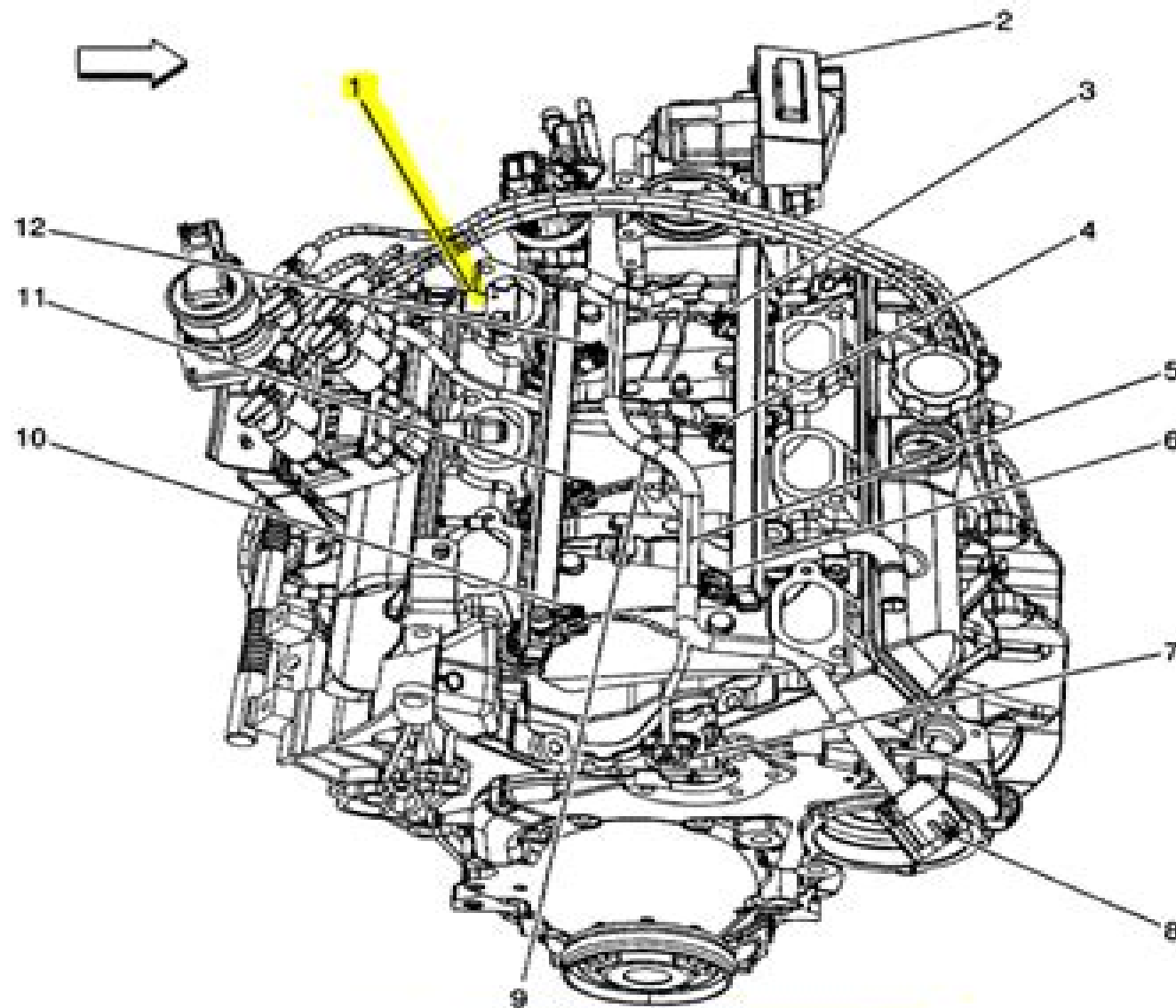
Fig 2: Engine Assembly (3.5L)
